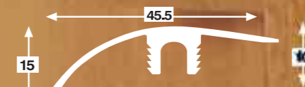
BHR 15 RAMP
