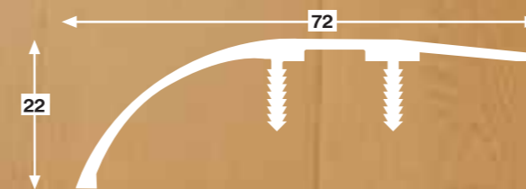
NFR3 22 RAMP
